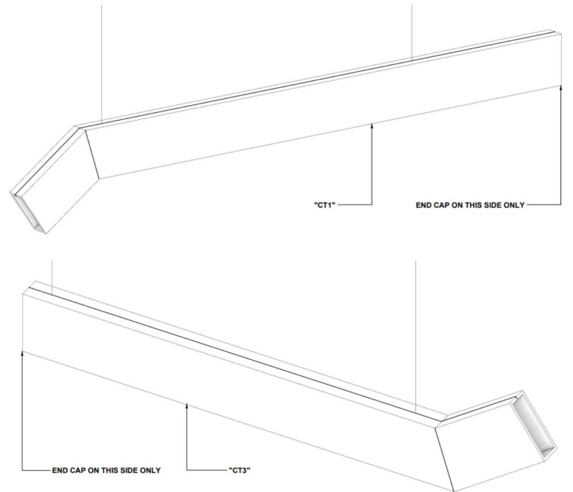
ASSEMBLED "CT1" & "CT3" NTS, FOR REPRESENTATION ONLY
