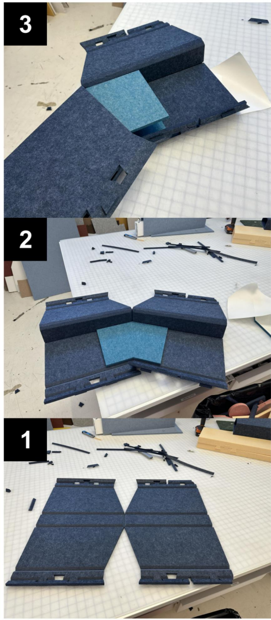
ASSEMBLY, "CT3" NTS, FOR REPRESENTATION ONLY
