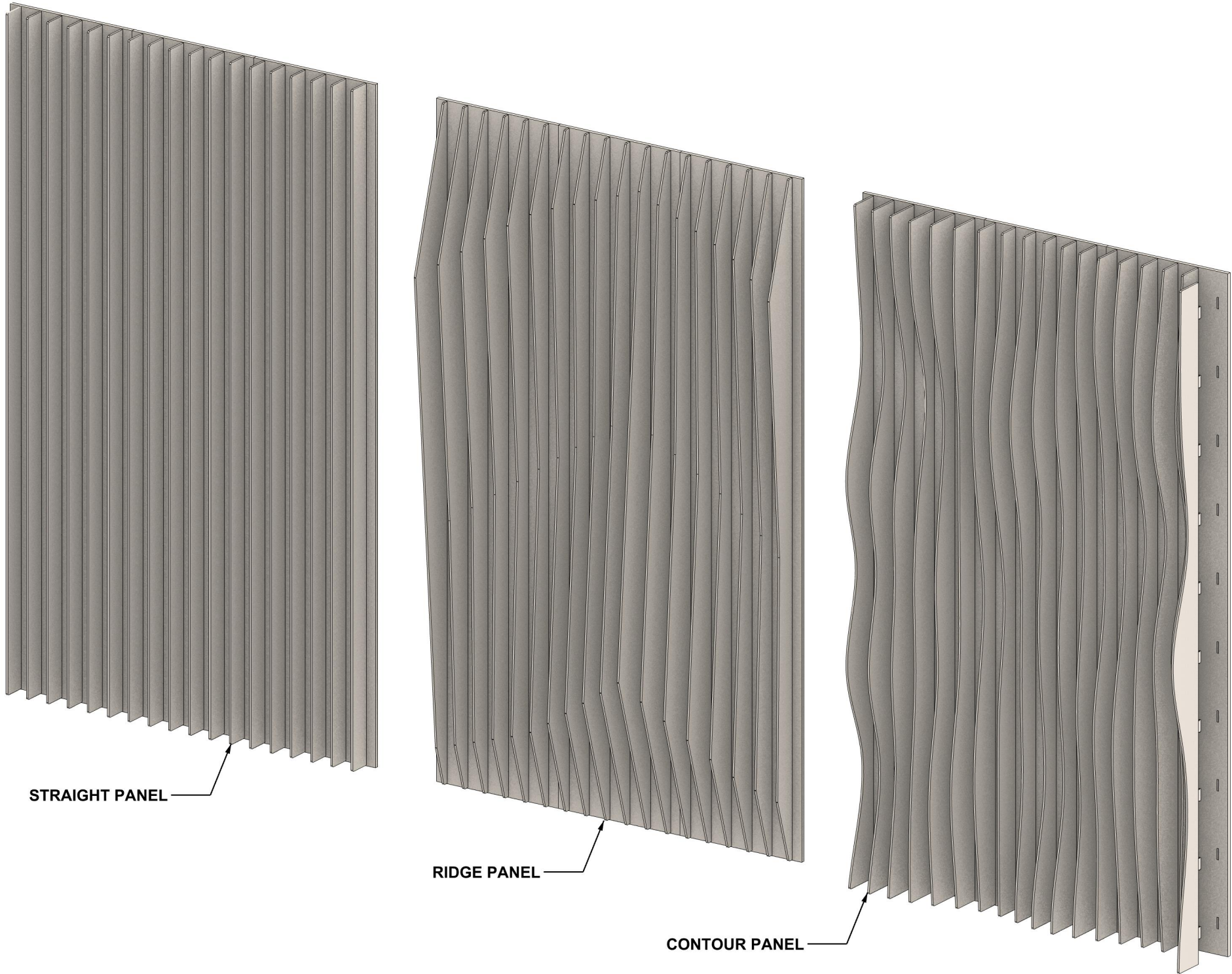
PRODUCT DEVELOPMENT - 9MM BAFFLE WALL (MASSING FROM SCRIPT OUTPUT) NTS
