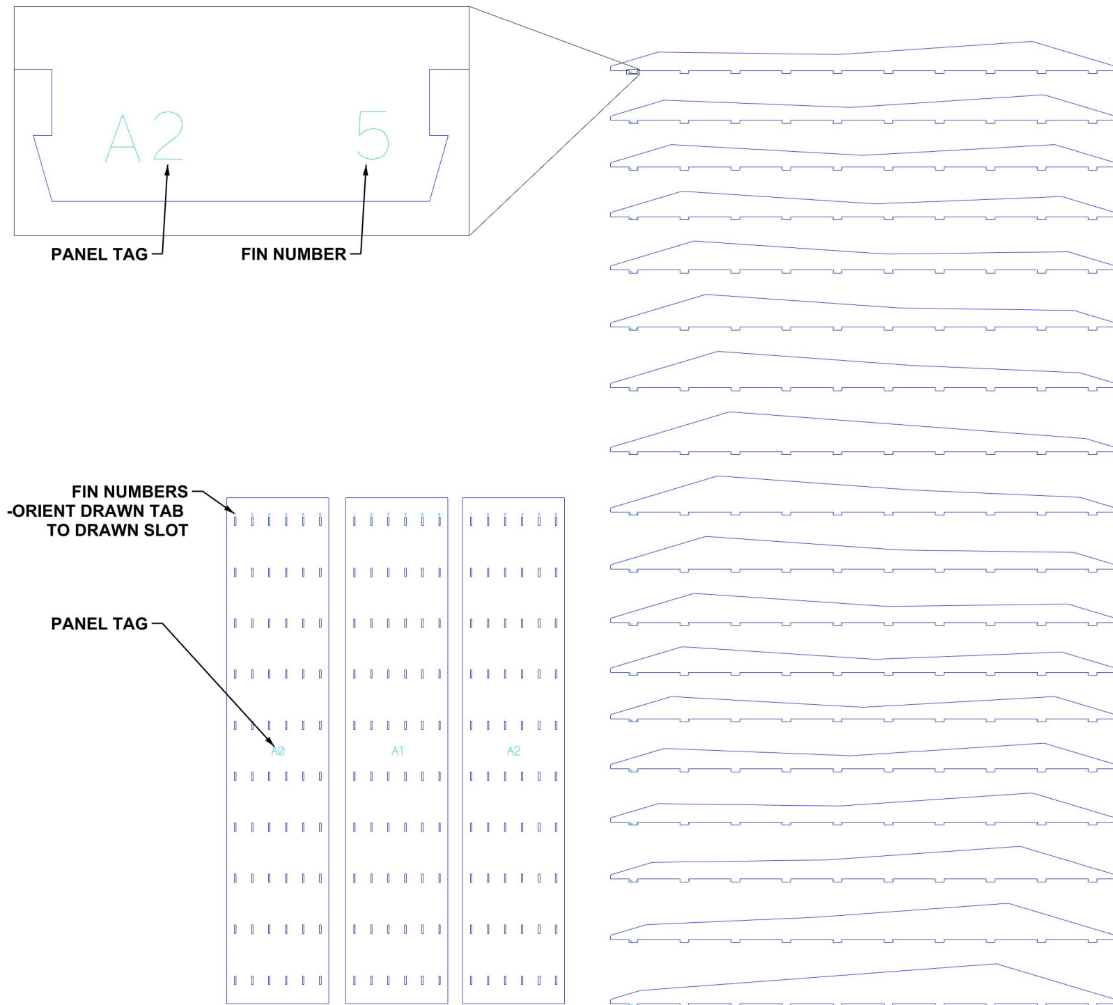
CONTOUR WALL OUTPUTS (CUTFILES) NTS 01
