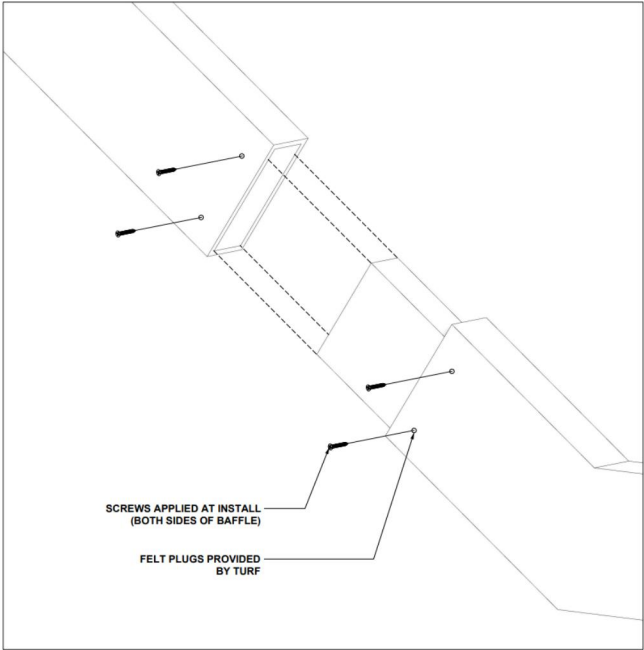
TENON DETAIL, FOLDED CUSTOM NTS 03
