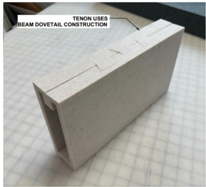
ASSEMBLED FOLDED TENON NTS, FOR REPRESENTATION ONLY
