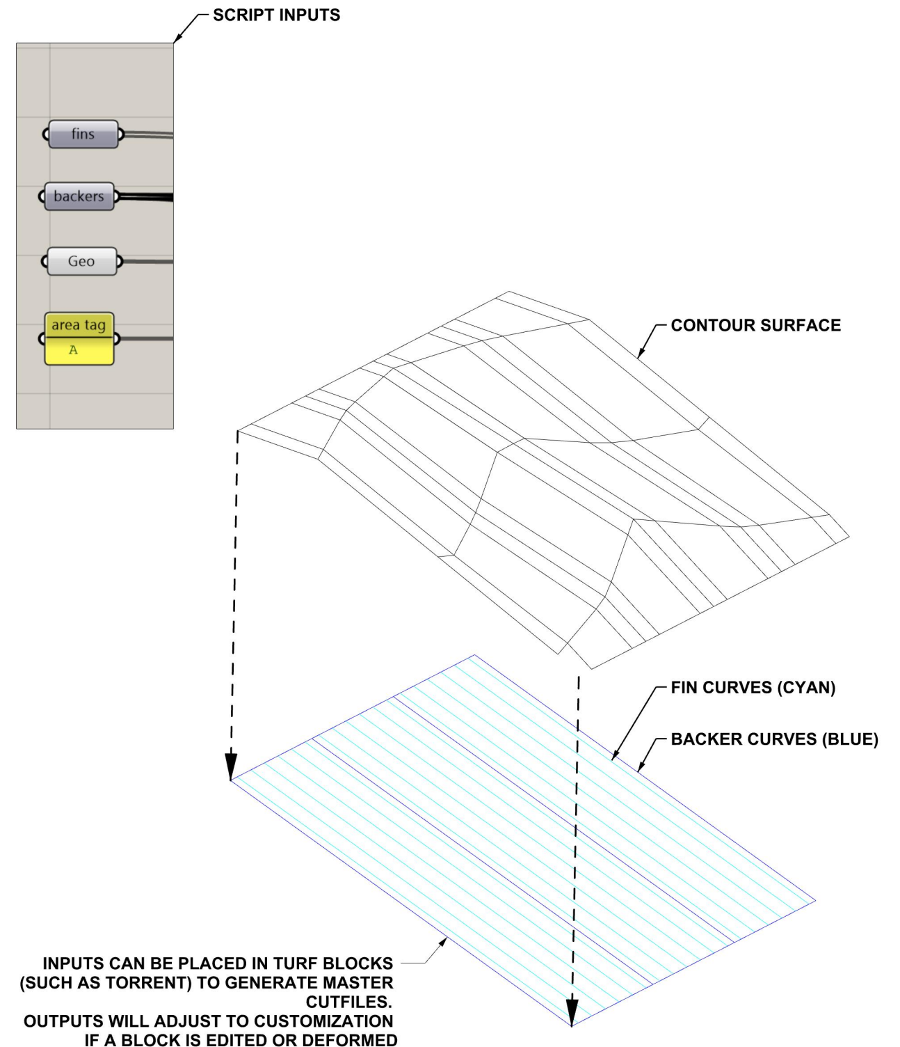
CONTOUR WALL INPUTS NTS 01
