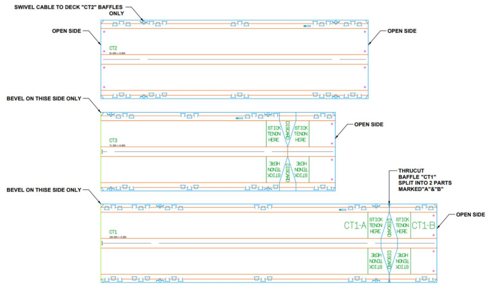
CUTFILES "CT1" - "CT3" NTS, FOR REPRESENTATION ONLY
